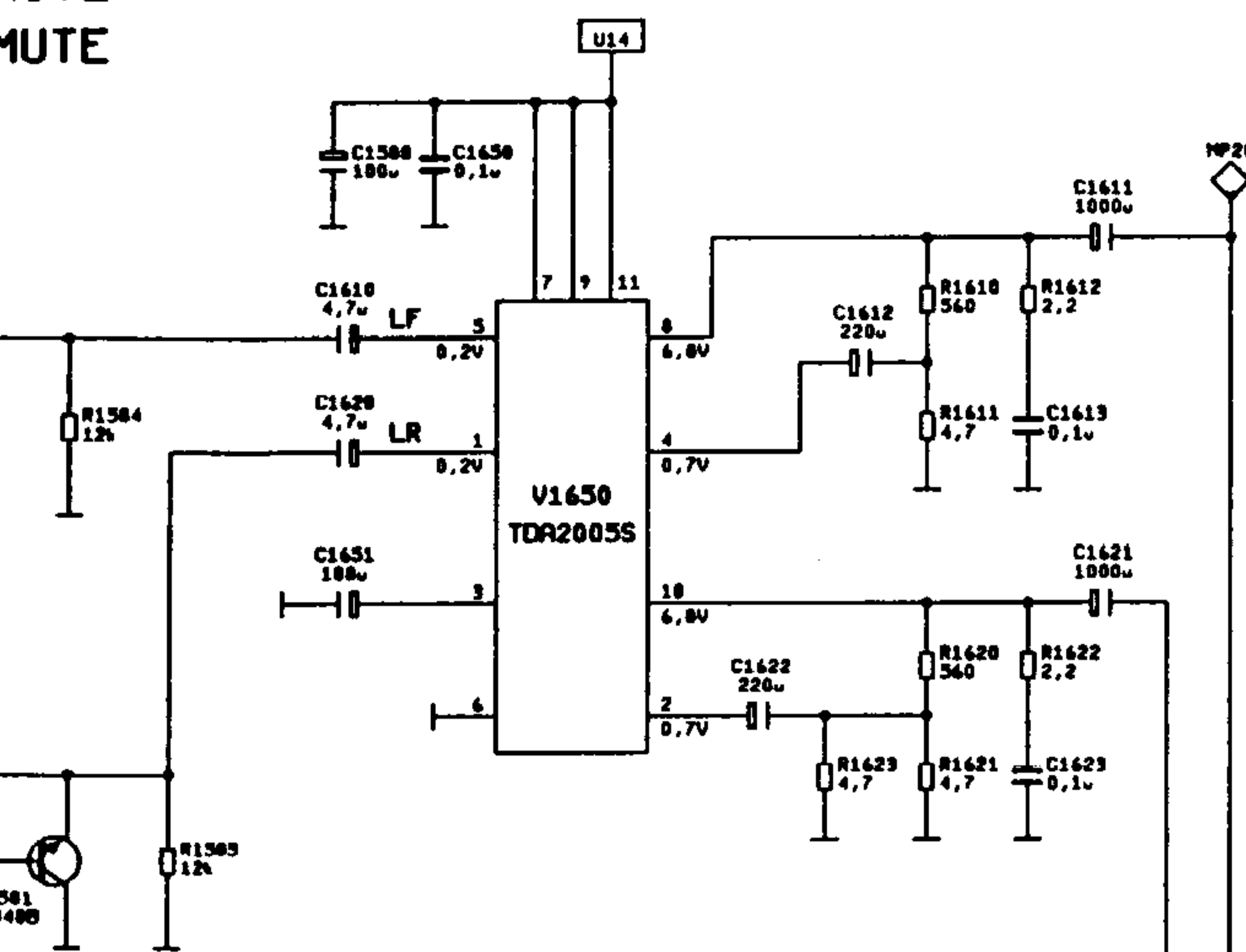
NF-ENDSTUFE AF-AMPLIFIER
